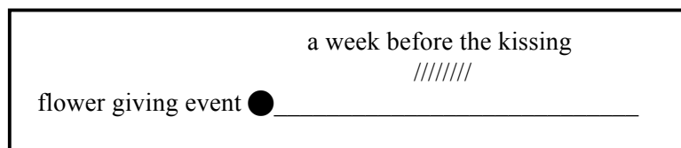
Figure 4: Wrong prediction
